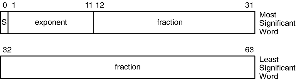
Figure 2-2 IEEE Double-Precision Format
