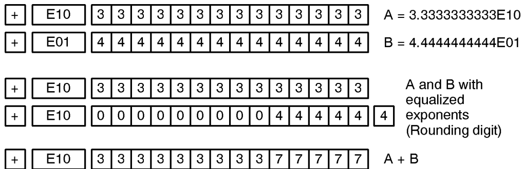
Figure 3-2 Adding Values with Very Different Magnitudes
