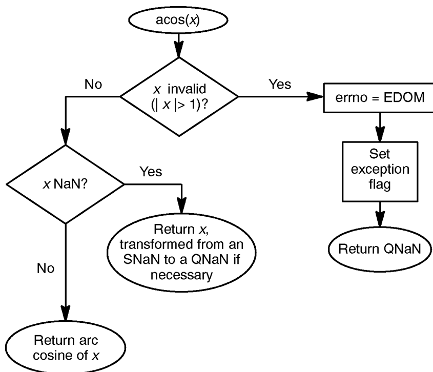
Figure 4-2 C Math Library Error Handling for the acos Function
