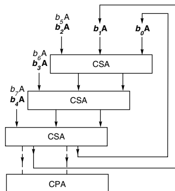
Figure H.28 Multipass array multiplier. Multiplies two 8-bit numbers with about half the hardware that would be used in a one-pass design like that of Figure H.27. At the end of the second pass, the bits flow into the CPA. The inputs used in the first pass are marked in bold.
