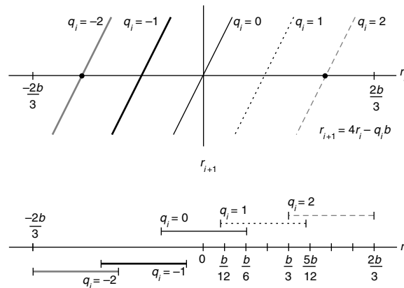
Figure H.33 Quotient selection for radix-4 division with quotient digits -2, -1, 0, 1, 2 .
