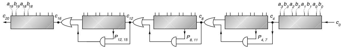
Figure H.19 Carry-skip adder. This is a 20-bit carry-skip adder ( n = 20 ) with each block 4-bits wide ( k = 4 ).
