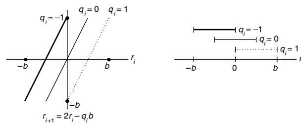
Figure H.32 Quotient selection for radix-2 division. The x -axis represents the i th remainder, which is the quantity in the (P, A) register pair. The y -axis shows the value of the remainder after one additional divide step. Each bar on the right-hand graph gives the range of r_i values for which it is permissible to select the associated value of q_i .
