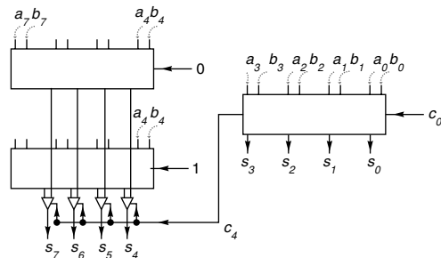
Figure H.20 Simple carry-select adder. At the same time that the sum of the low-order 4 bits is being computed, the high-order bits are being computed twice in parallel: once assuming that c_4 = 0 and once assuming c_4 = 1 .
