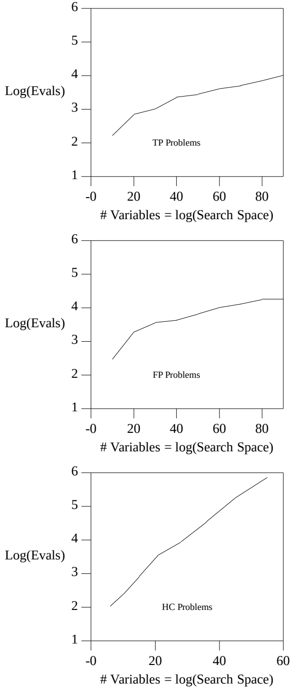
Figure 7: Summary Performance of GAs using AVE^2
