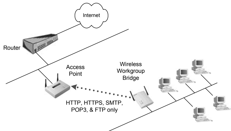
FIGURE 10.7 Protocol Filtering
