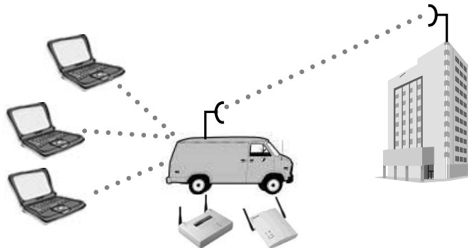
FIGURE 10.11 Man-in-the-middle attack
