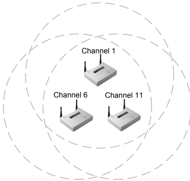
FIGURE 9.9 Co-location Throughput
