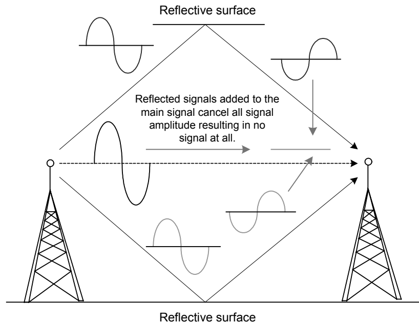
FIGURE 9.4 RF Signal Nulling
