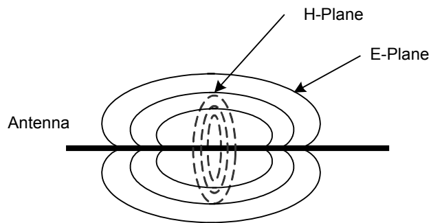
FIGURE 5.13 E-planes and H-planes
