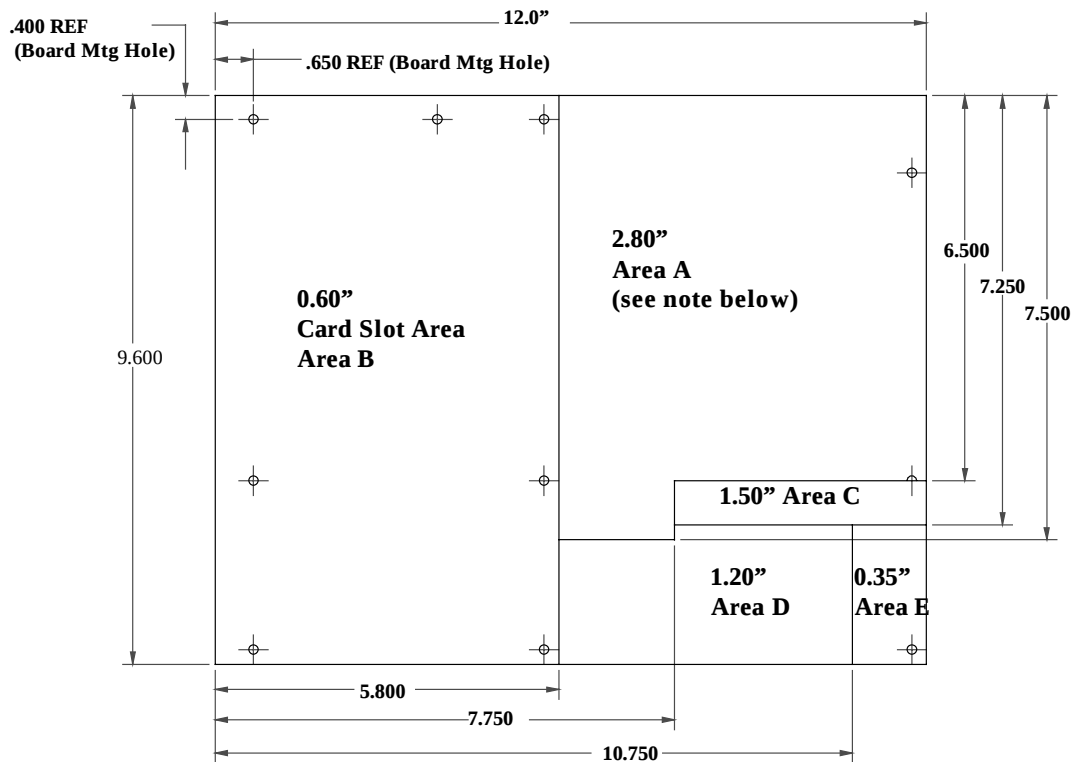
Figure 7. ATX Motherboard Maximum Component Height Restrictions
