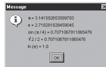
Figure 6–5 Application com.eteks.test.ValeursMathematiques
