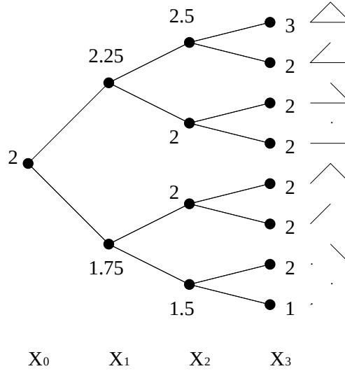
Figure 7.1: The edge exposure process with n = 3 where the edges are exposed in the order “bottom, left, right”. The values \chi_i(H) are given by tracing from the central node to the leaf labeled H .
