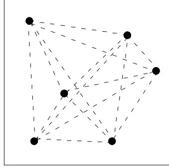
Figure 3.1: 6 points determine 20 triangles
